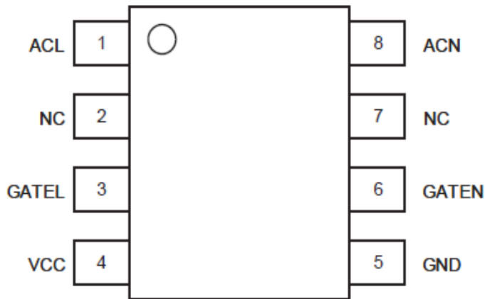
SO8 (Top View)
